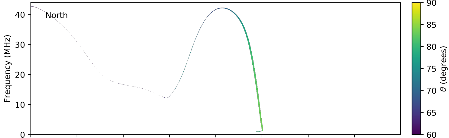
expres_earth_jupiter_io_jrm09_lossc-wid1deg_3kev_20100330_v01.cdf
