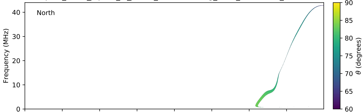
expres_earth_jupiter_io_jrm09_lossc-wid1deg_3kev_20100329_v01.cdf
