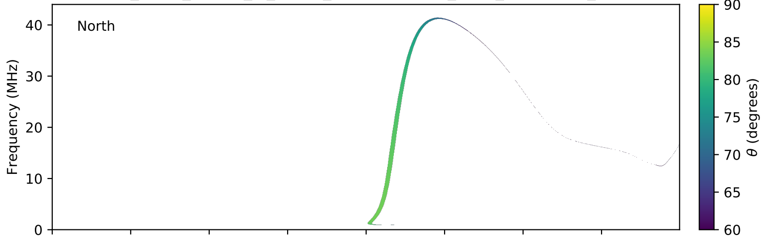
expres_earth_jupiter_io_jrm09_lossc-wid1deg_3kev_20100324_v01.cdf
