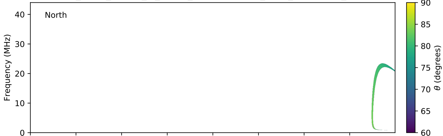
expres_earth_jupiter_io_jrm09_lossc-wid1deg_3kev_20100320_v01.cdf
