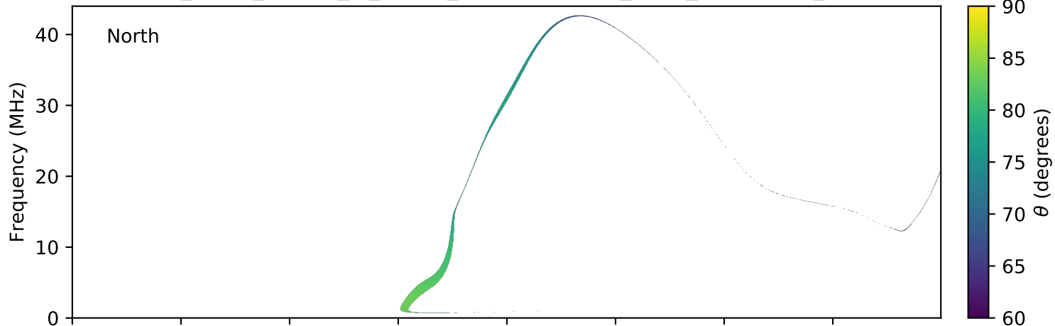
expres_earth_jupiter_io_jrm09_lossc-wid1deg_3kev_20100317_v01.cdf
