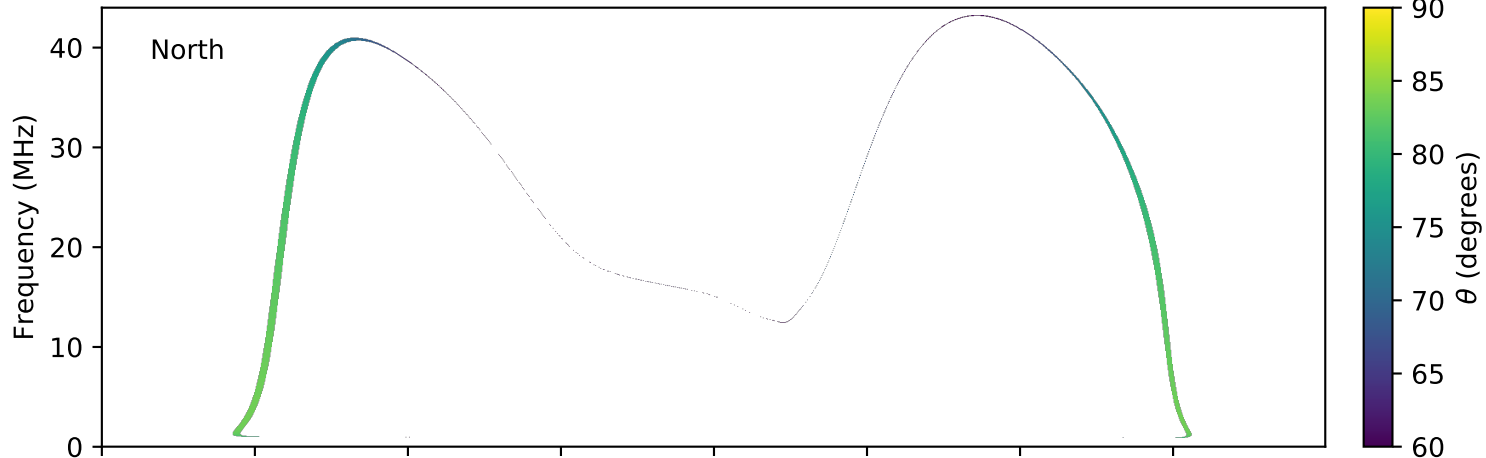
expres_earth_jupiter_io_jrm09_lossc-wid1deg_3kev_20100312_v01.cdf
