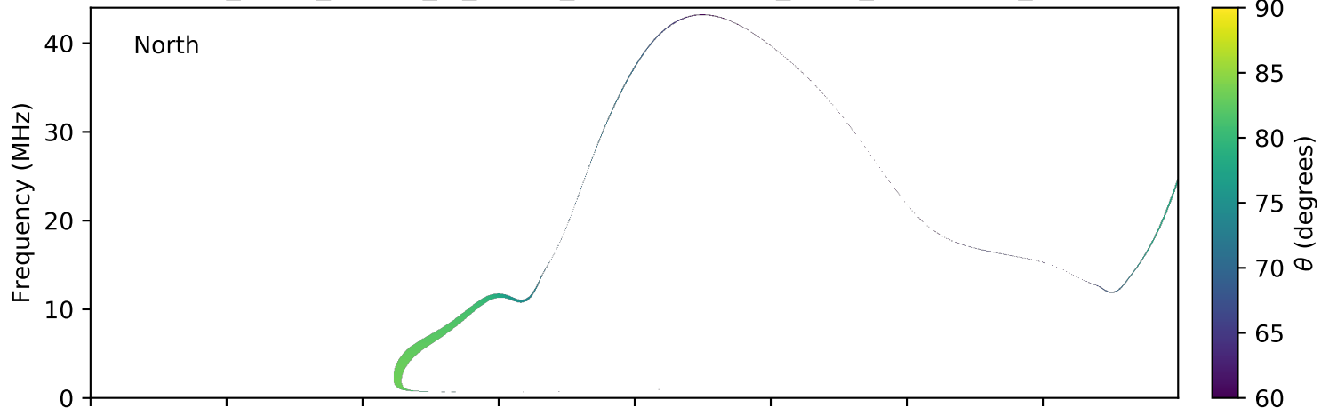
expres_earth_jupiter_io_jrm09_lossc-wid1deg_3kev_20100310_v01.cdf
