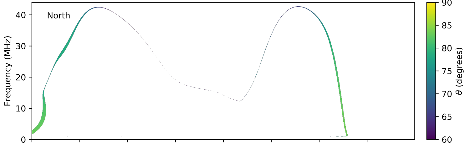
expres_earth_jupiter_io_jrm09_lossc-wid1deg_3kev_20100305_v01.cdf
