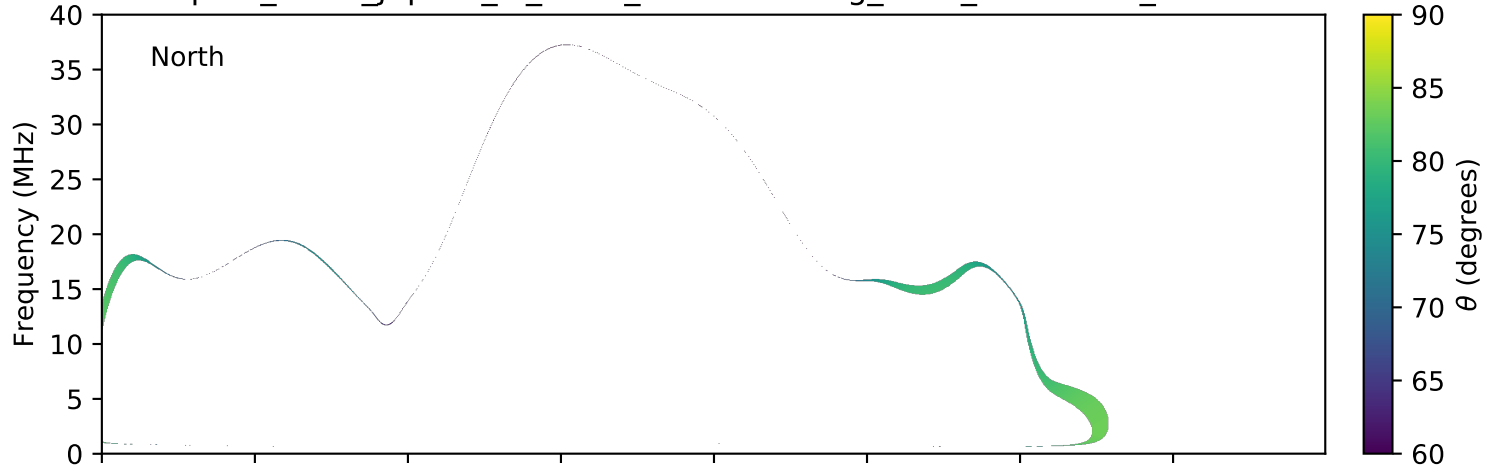
expres_earth_jupiter_io_isaac_lossc-wid1deg_3kev_20100328_v01.cdf
