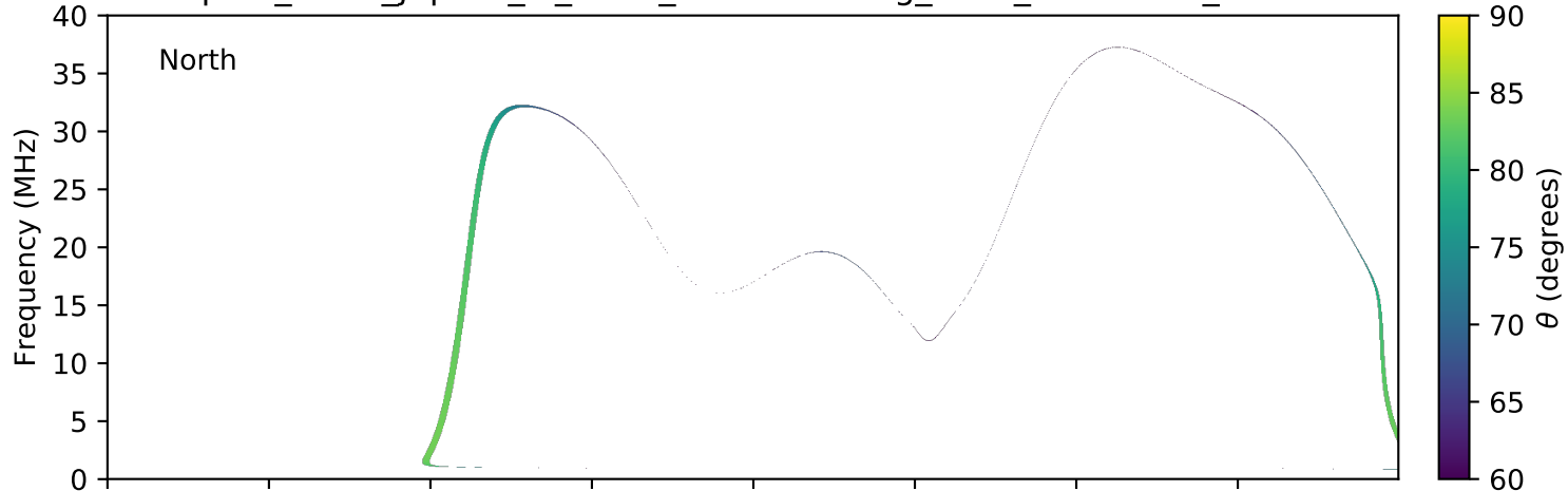
expres_earth_jupiter_io_isaac_lossc-wid1deg_3kev_20100326_v01.cdf
