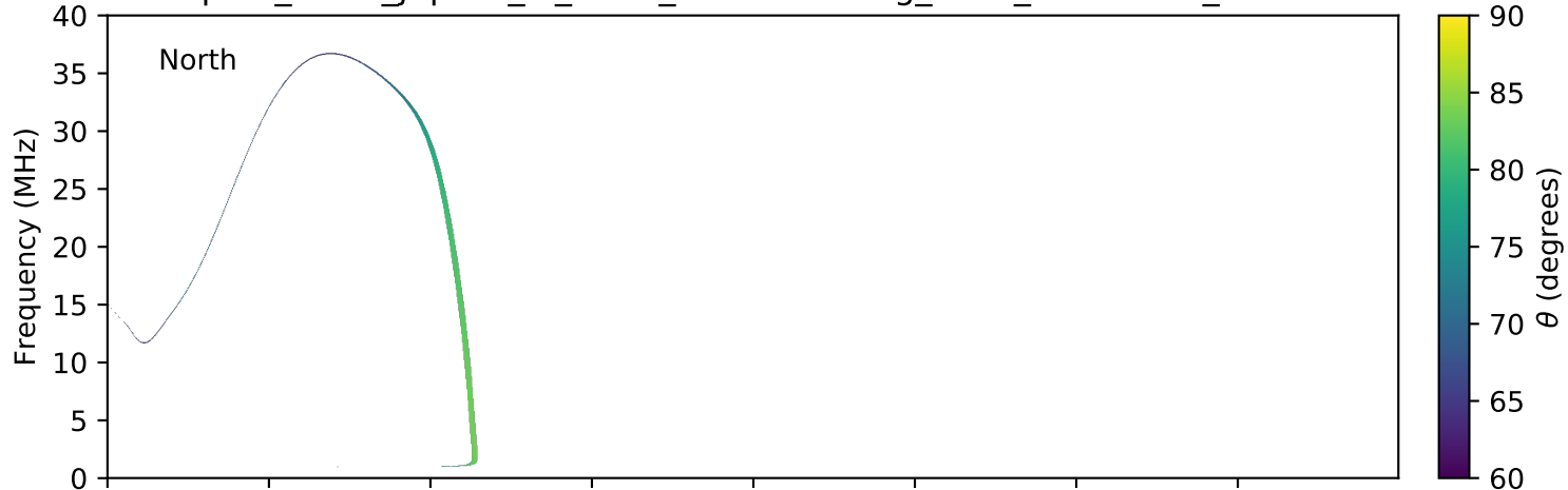
expres_earth_jupiter_io_isaac_lossc-wid1deg_3kev_20100325_v01.cdf
