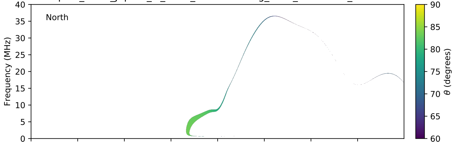
expres_earth_jupiter_io_isaac_lossc-wid1deg_3kev_20100324_v01.cdf
