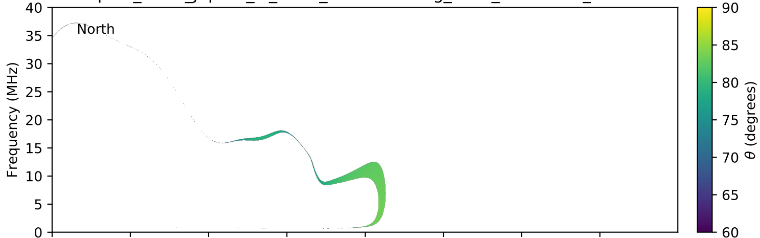
expres_earth_jupiter_io_isaac_lossc-wid1deg_3kev_20100323_v01.cdf
