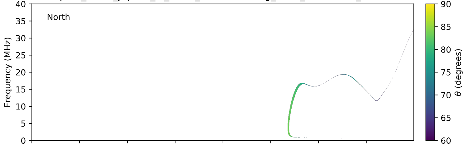
expres_earth_jupiter_io_isaac_lossc-wid1deg_3kev_20100322_v01.cdf
