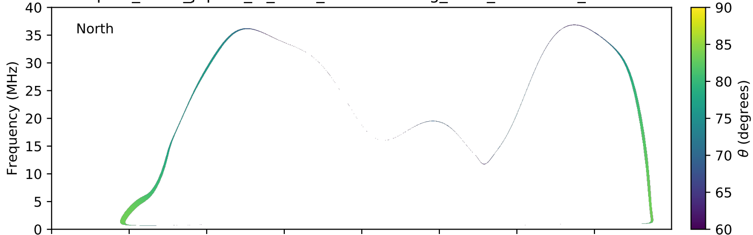
expres_earth_jupiter_io_isaac_lossc-wid1deg_3kev_20100319_v01.cdf
