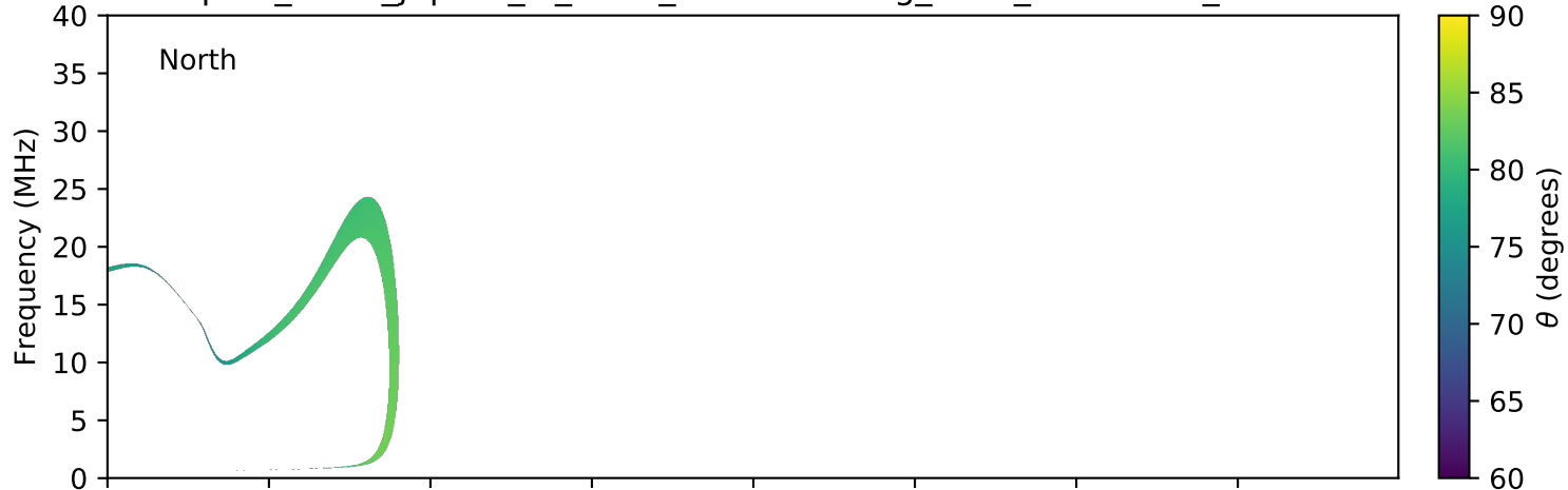
expres_earth_jupiter_io_isaac_lossc-wid1deg_3kev_20100318_v01.cdf
