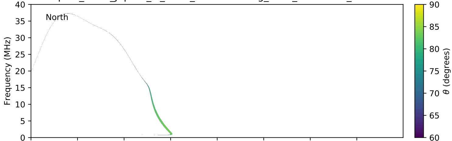
expres_earth_jupiter_io_isaac_lossc-wid1deg_3kev_20100316_v01.cdf
