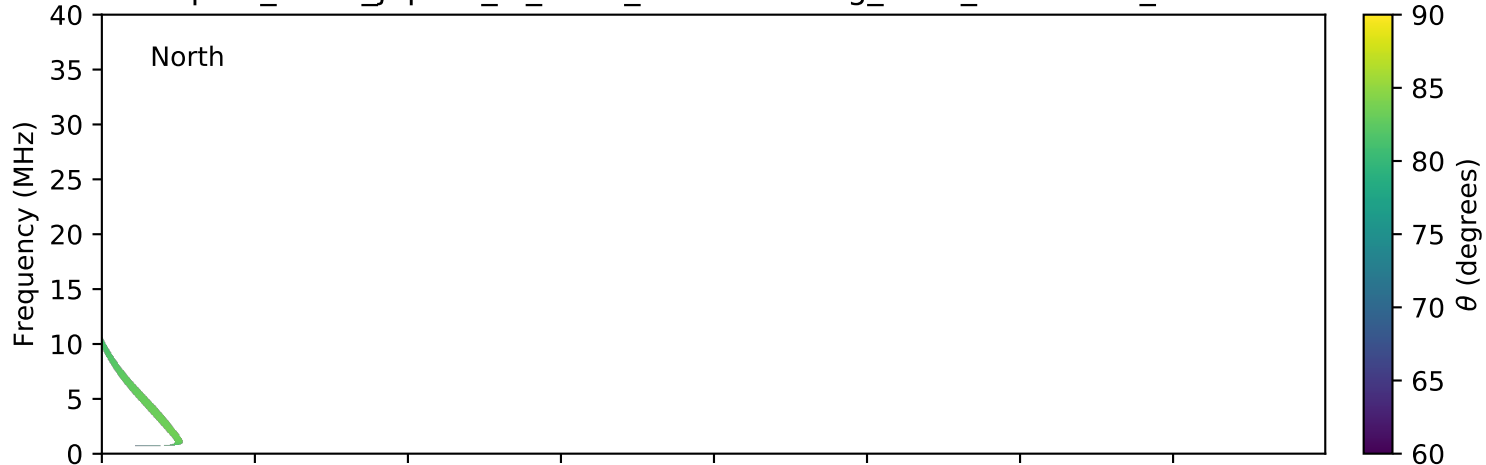
expres_earth_jupiter_io_isaac_lossc-wid1deg_3kev_20100311_v01.cdf
