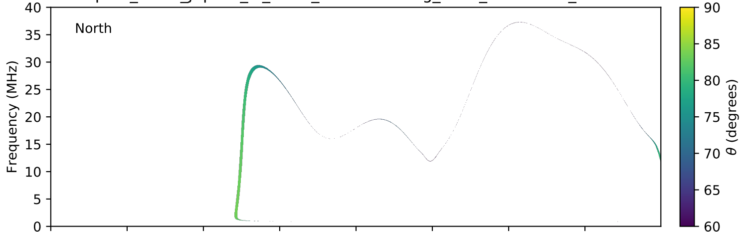
expres_earth_jupiter_io_isaac_lossc-wid1deg_3kev_20100310_v01.cdf
