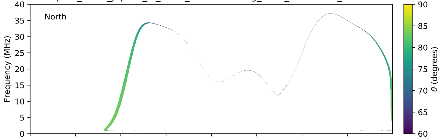
expres_earth_jupiter_io_isaac_lossc-wid1deg_3kev_20100303_v01.cdf
