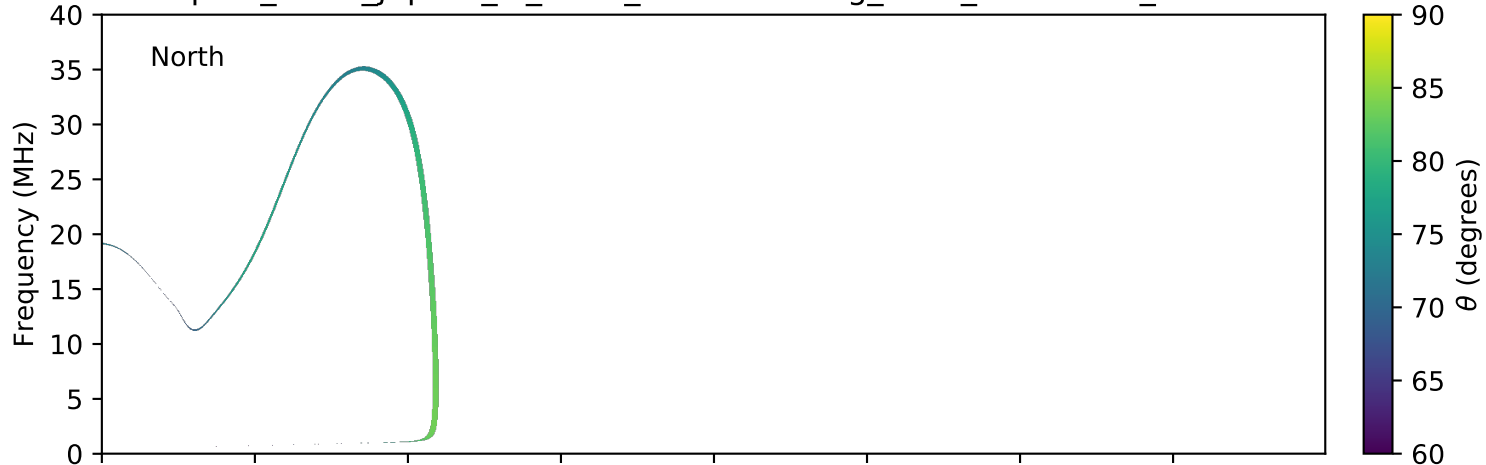
expres_earth_jupiter_io_isaac_lossc-wid1deg_3kev_20100302_v01.cdf
