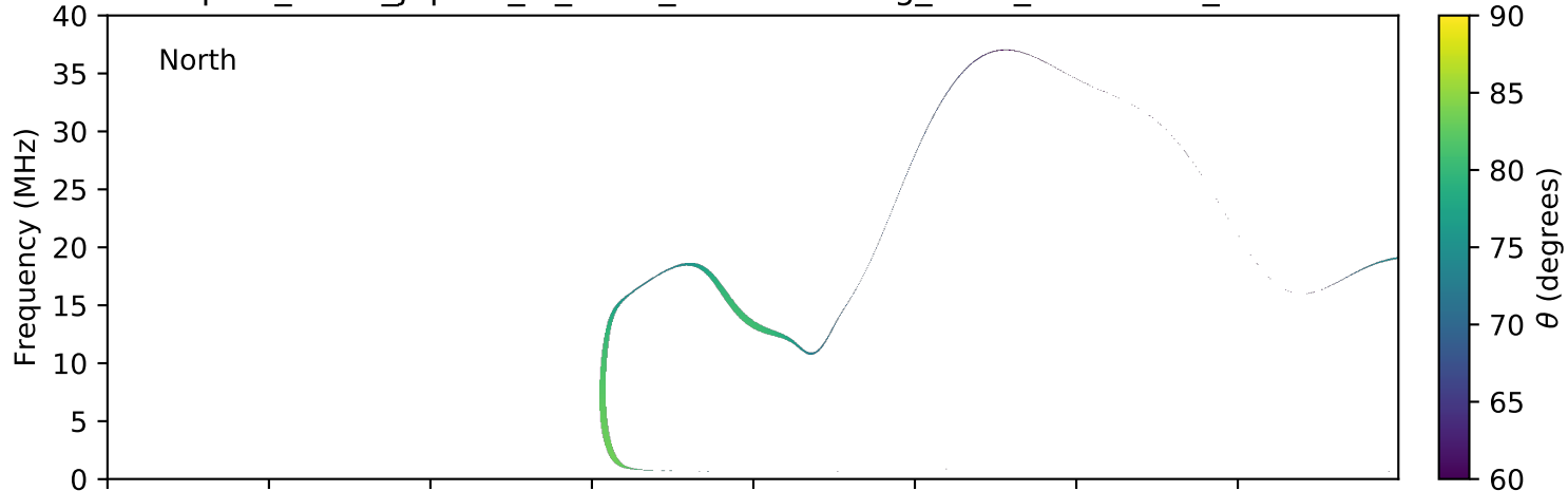
expres_earth_jupiter_io_isaac_lossc-wid1deg_3kev_20100301_v01.cdf
