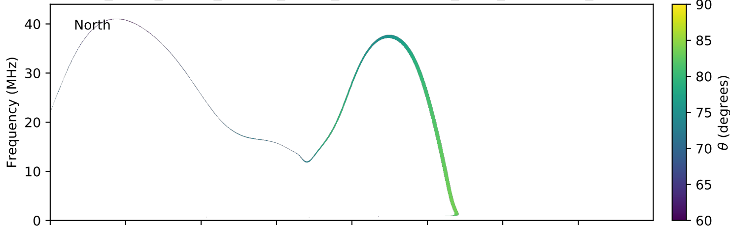
expres_earth_jupiter_europa_jrm09_lossc-wid1deg_3kev_20100325_v01.cdf
