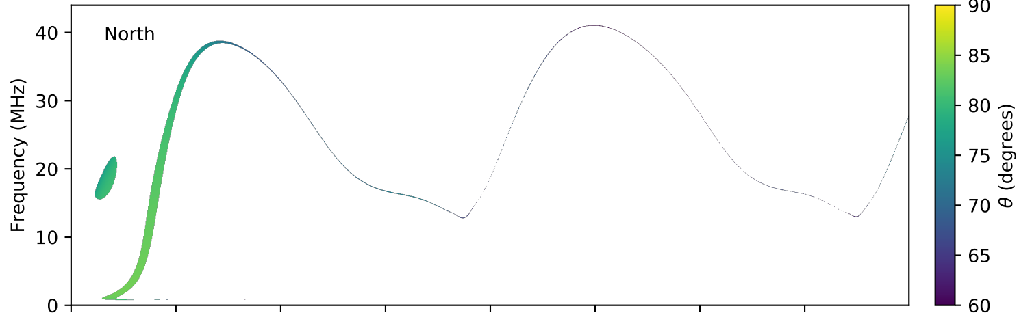
expres_earth_jupiter_europa_jrm09_lossc-wid1deg_3kev_20100317_v01.cdf
