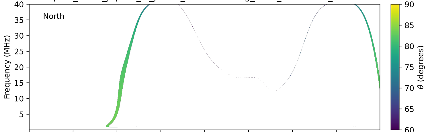
expres_earth_jupiter_io_jrm33_lossc-wid1deg_3kev_20100208_v11.cdf
