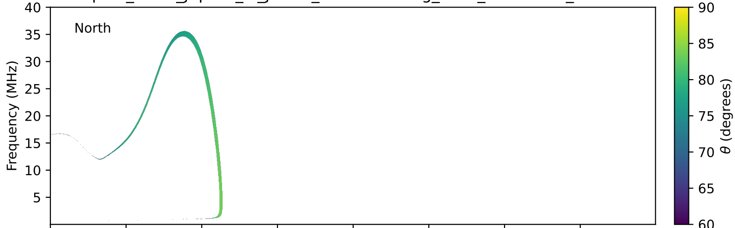
expres_earth_jupiter_io_jrm33_lossc-wid1deg_3kev_20100207_v11.cdf
