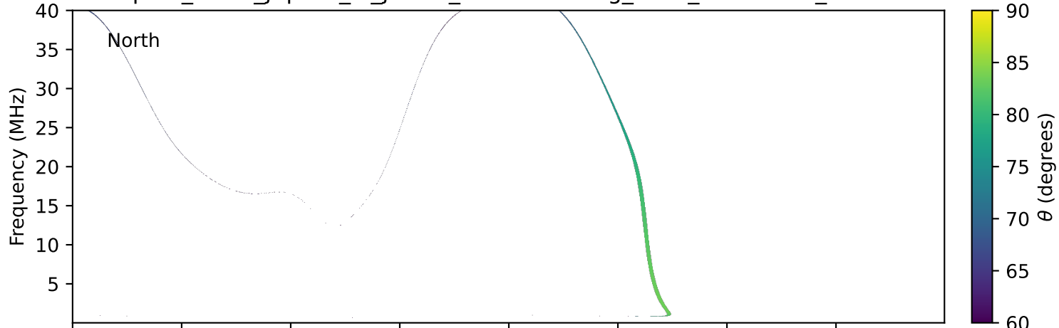
expres_earth_jupiter_io_jrm33_lossc-wid1deg_3kev_20100203_v11.cdf
