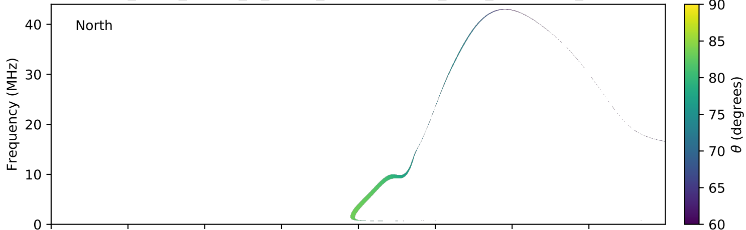
expres_earth_jupiter_io_jrm09_lossc-wid1deg_3kev_20100213_v01.cdf
