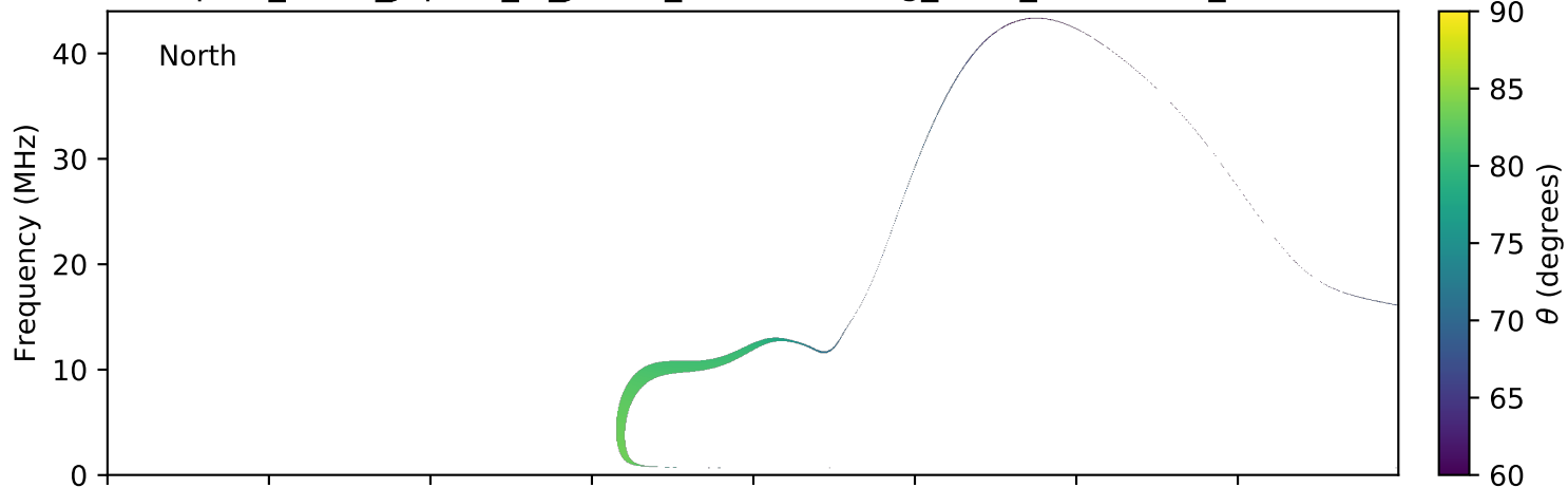
expres_earth_jupiter_io_jrm09_lossc-wid1deg_3kev_20100206_v01.cdf
