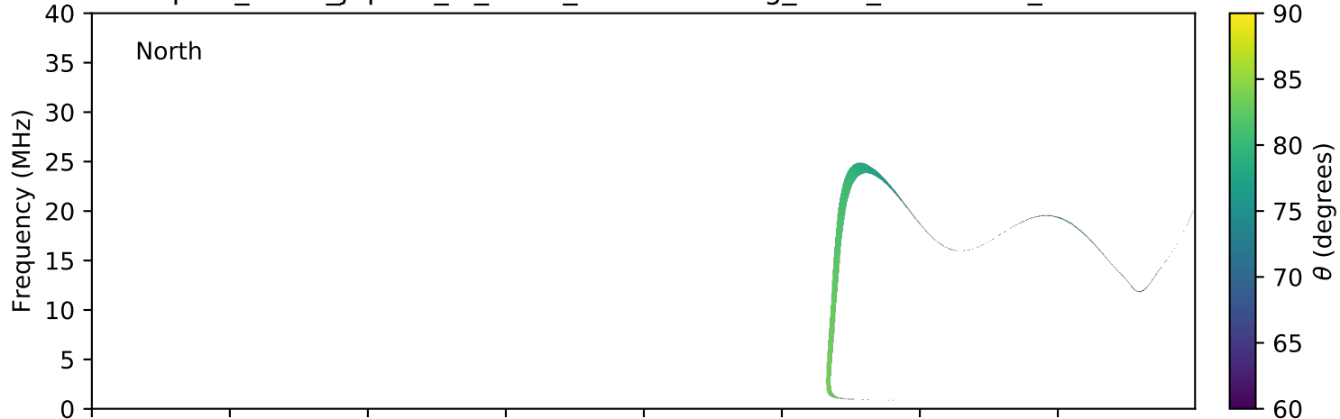
expres_earth_jupiter_io_isaac_lossc-wid1deg_3kev_20100227_v01.cdf
