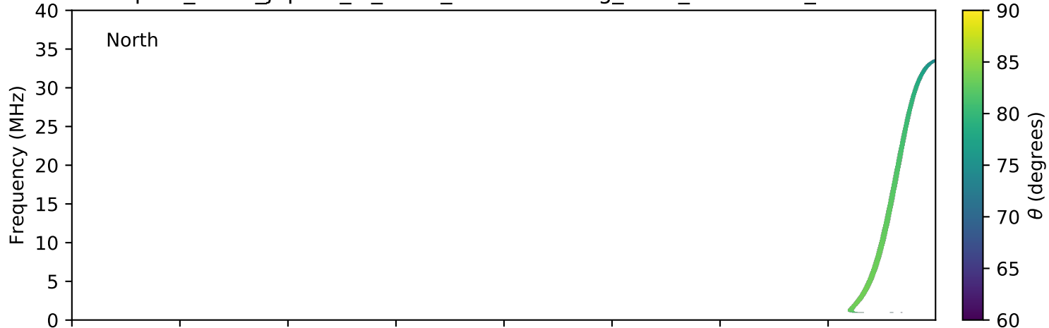
expres_earth_jupiter_io_isaac_lossc-wid1deg_3kev_20100225_v01.cdf
