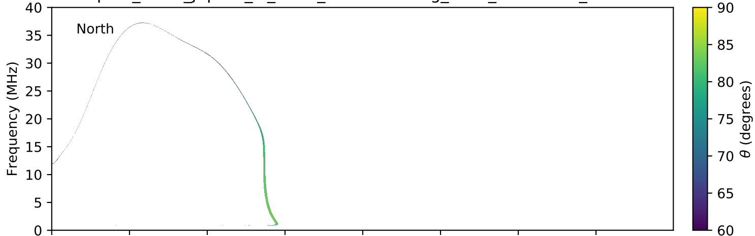
expres_earth_jupiter_io_isaac_lossc-wid1deg_3kev_20100221_v01.cdf
