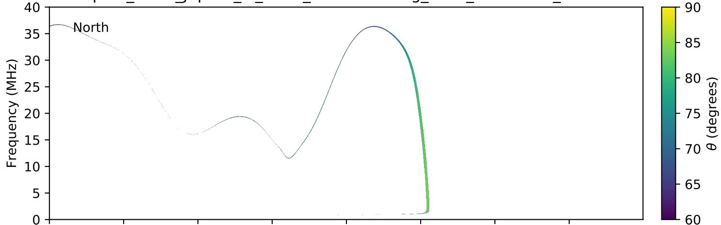
expres_earth_jupiter_io_isaac_lossc-wid1deg_3kev_20100219_v01.cdf
