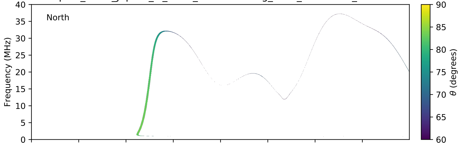
expres_earth_jupiter_io_isaac_lossc-wid1deg_3kev_20100215_v01.cdf
