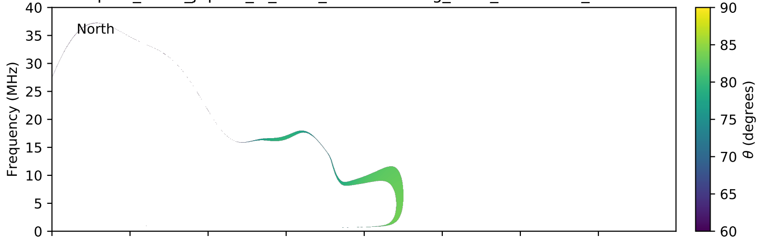
expres_earth_jupiter_io_isaac_lossc-wid1deg_3kev_20100212_v01.cdf
