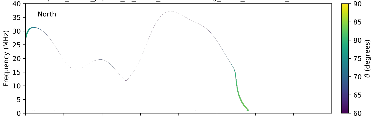
expres_earth_jupiter_io_isaac_lossc-wid1deg_3kev_20100210_v01.cdf
