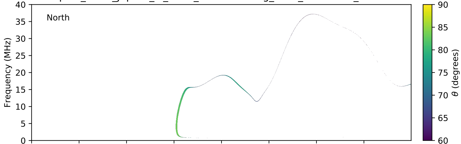
expres_earth_jupiter_io_isaac_lossc-wid1deg_3kev_20100206_v01.cdf
