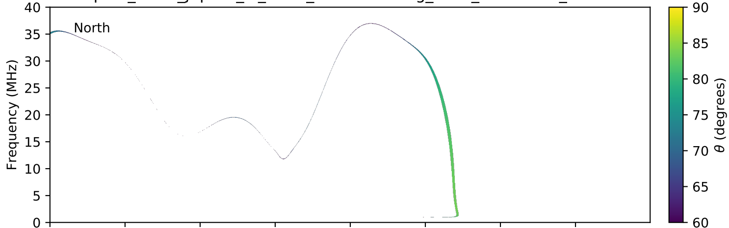
expres_earth_jupiter_io_isaac_lossc-wid1deg_3kev_20100203_v01.cdf
