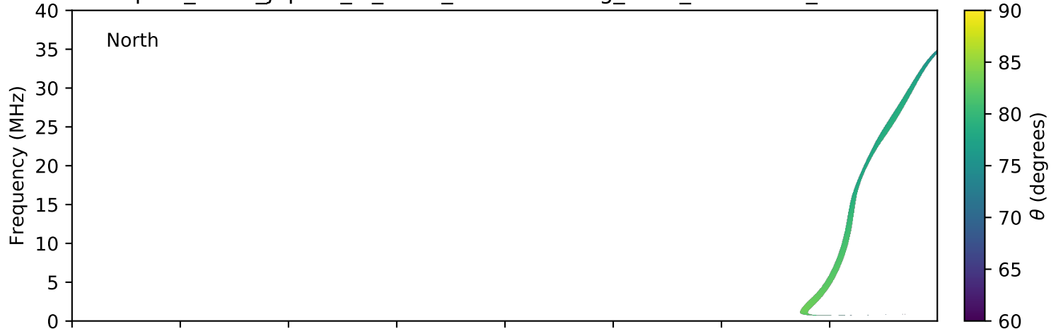
expres_earth_jupiter_io_isaac_lossc-wid1deg_3kev_20100202_v01.cdf
