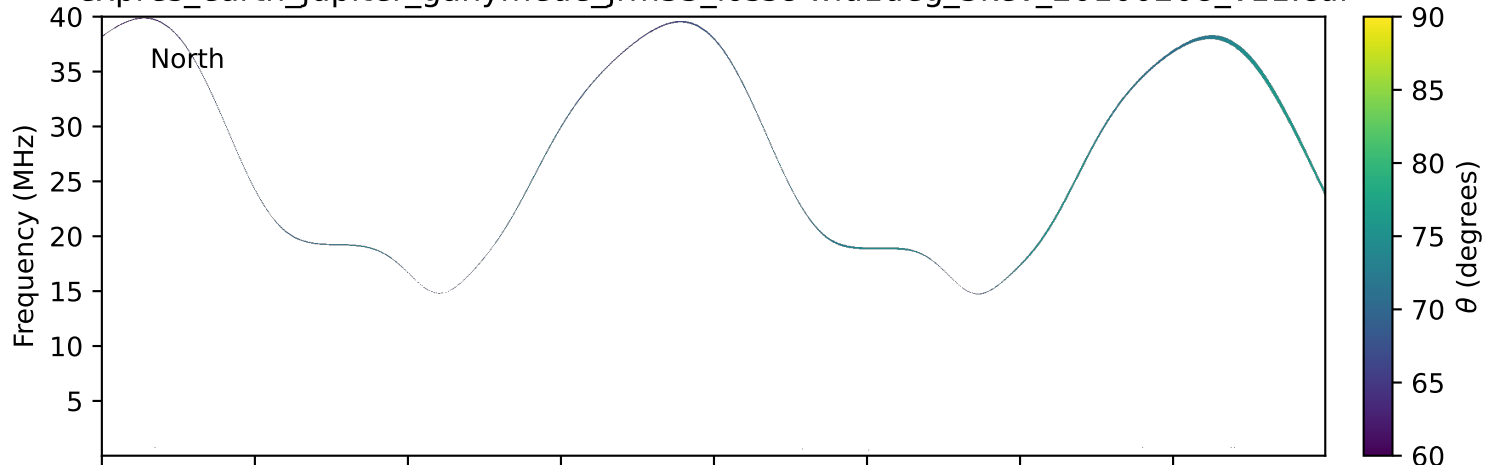
expres_earth_jupiter_ganymede_jrm33_lossc-wid1deg_3kev_20100208_v11.cdf
