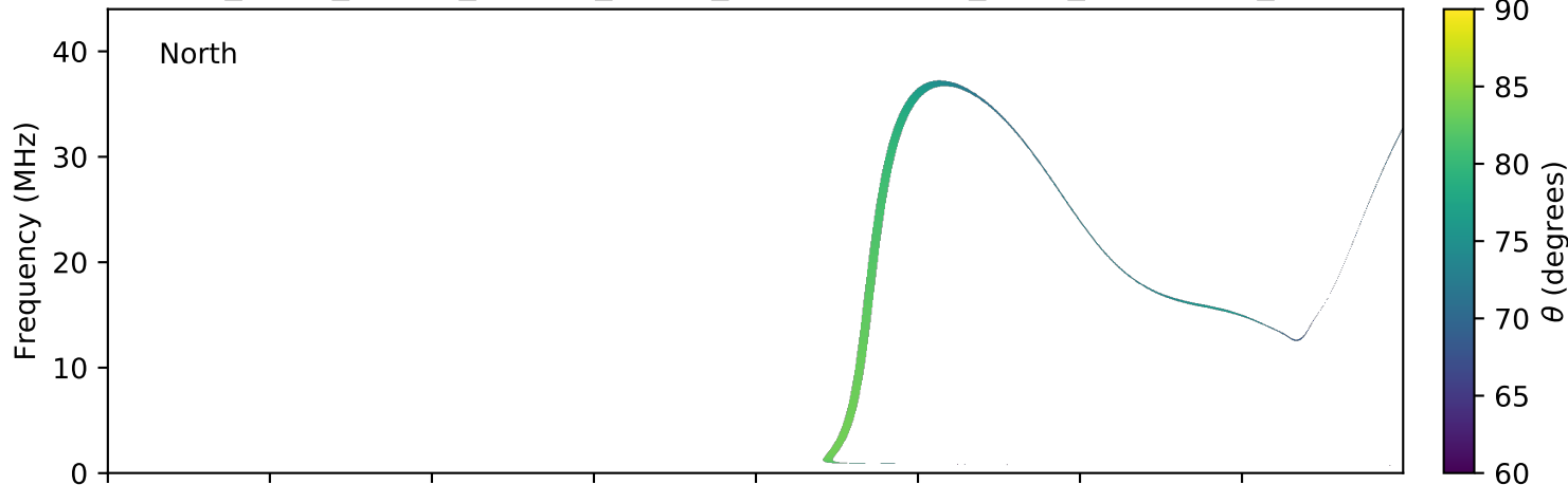
expres_earth_jupiter_europa_jrm09_lossc-wid1deg_3kev_20100216_v01.cdf
