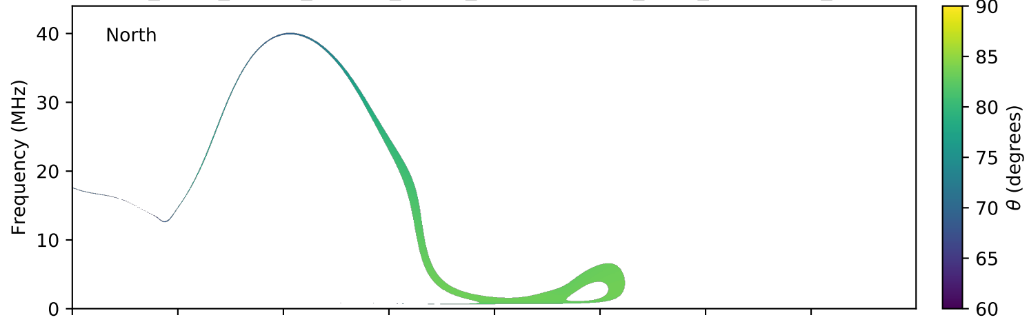
expres_earth_jupiter_europa_jrm09_lossc-wid1deg_3kev_20100214_v01.cdf
