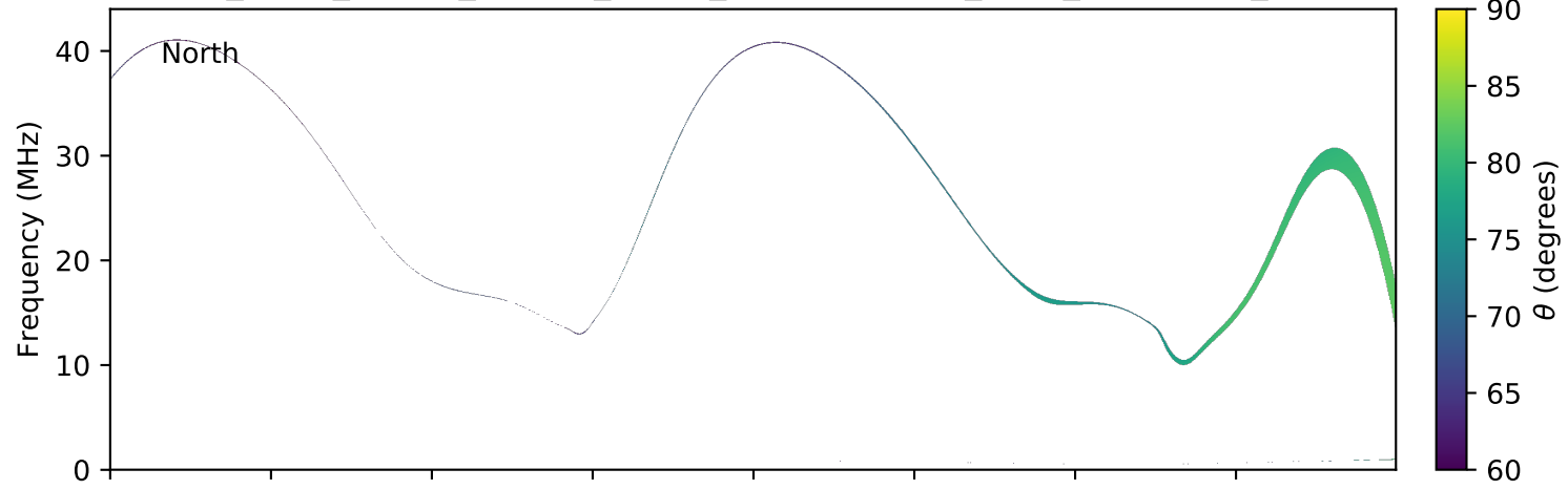
expres_earth_jupiter_europa_jrm09_lossc-wid1deg_3kev_20100210_v01.cdf
