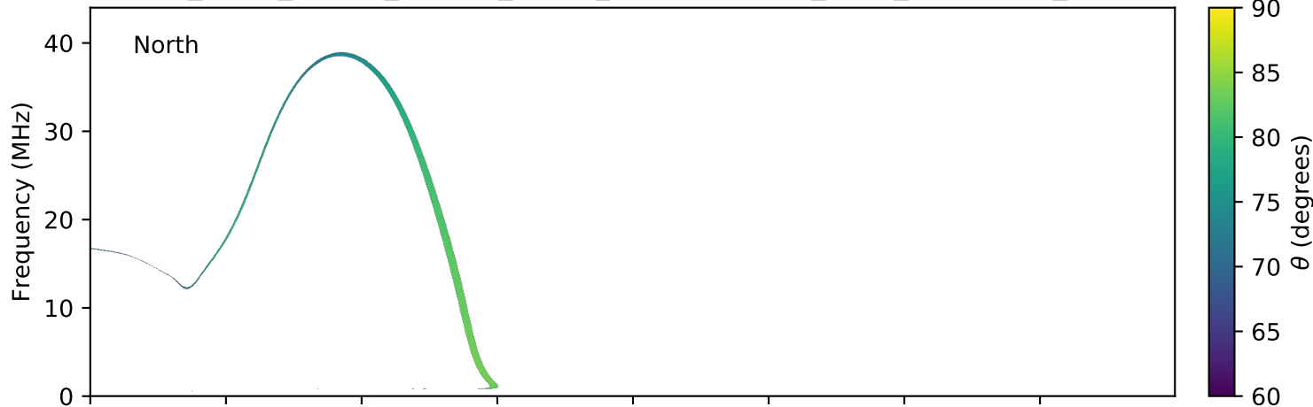
expres_earth_jupiter_europa_jrm09_lossc-wid1deg_3kev_20100207_v01.cdf
