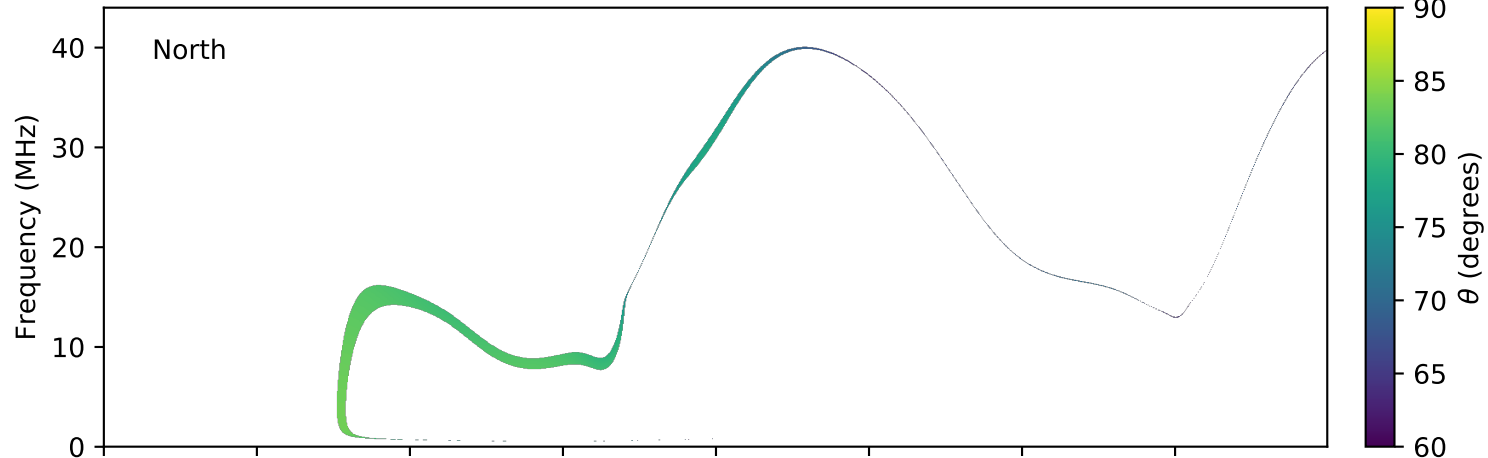
expres_earth_jupiter_europa_jrm09_lossc-wid1deg_3kev_20100202_v01.cdf
