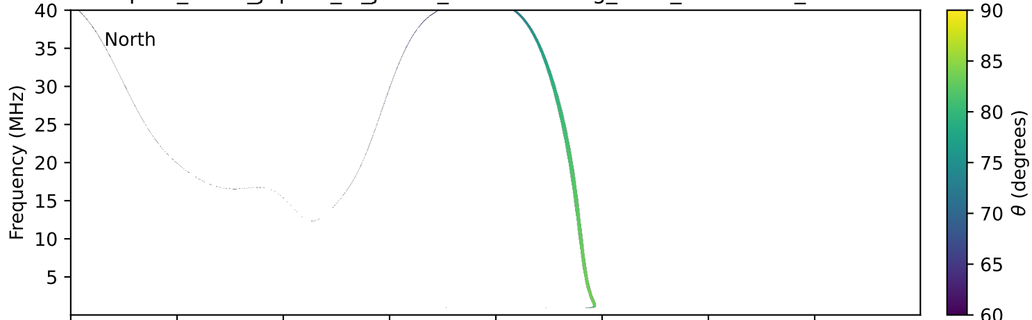
expres_earth_jupiter_io_jrm33_lossc-wid1deg_3kev_20100127_v11.cdf
