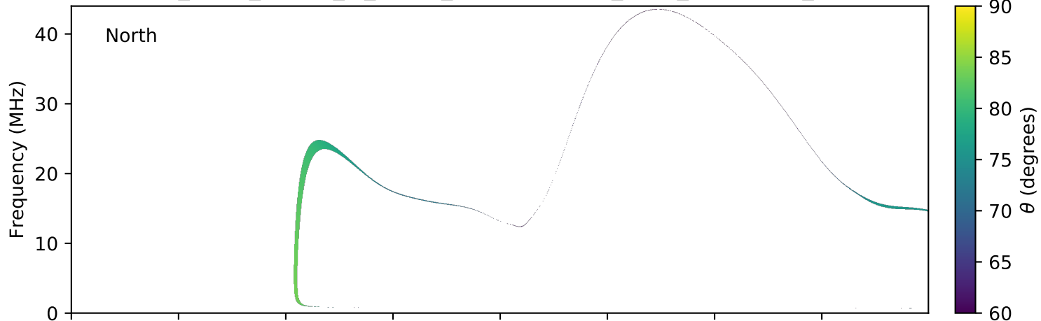
expres_earth_jupiter_io_jrm09_lossc-wid1deg_3kev_20100123_v01.cdf
