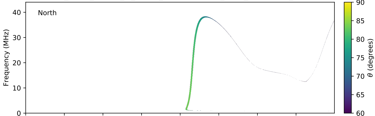
expres_earth_jupiter_io_jrm09_lossc-wid1deg_3kev_20100121_v01.cdf
