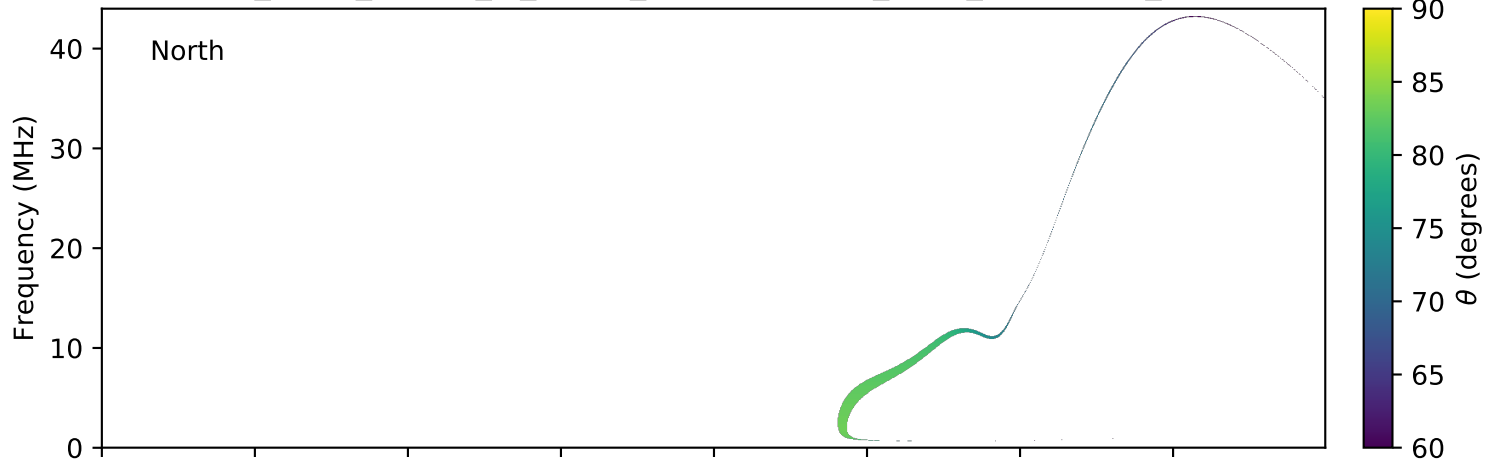
expres_earth_jupiter_io_jrm09_lossc-wid1deg_3kev_20100112_v01.cdf
