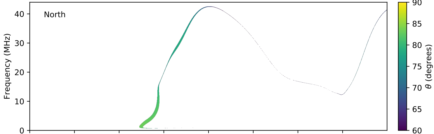
expres_earth_jupiter_io_jrm09_lossc-wid1deg_3kev_20100107_v01.cdf
